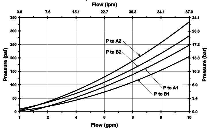
Pressure vs. Flow for LV Relief
