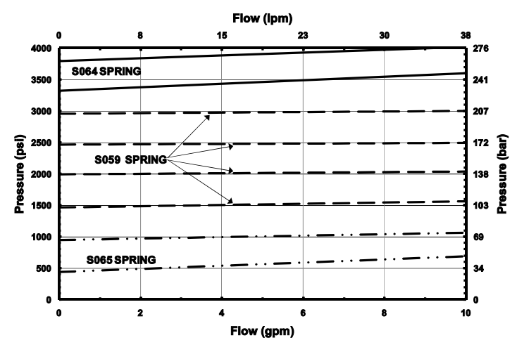
Pressure vs. Flow for LV Relief
