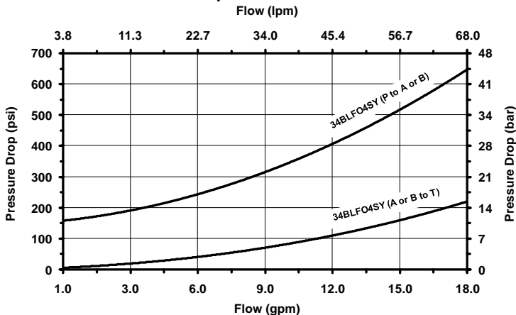
S34 Pressure Drop vs. Flow for 34BLF Sections
