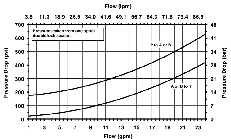
S36 Press. Drop vs. Flow for Double Lock Sect.
