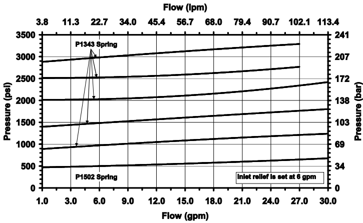
Pressure vs. Flow for Inlet Relief
