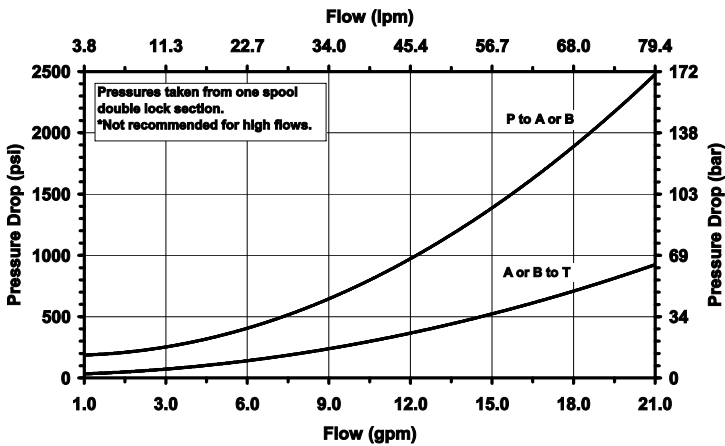
Press. Drop vs. Flow for Double Lock Sect.
