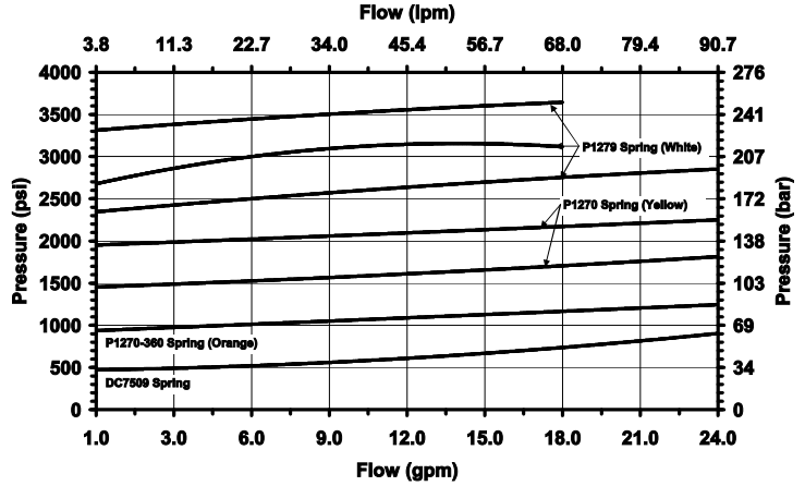
Pressure Drop vs. Flow for S36 Relief
