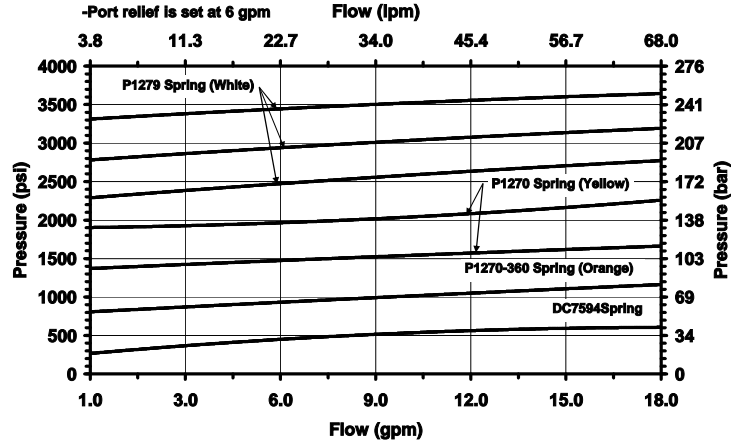
Pressure Drop vs. Flow for S34 Relief
