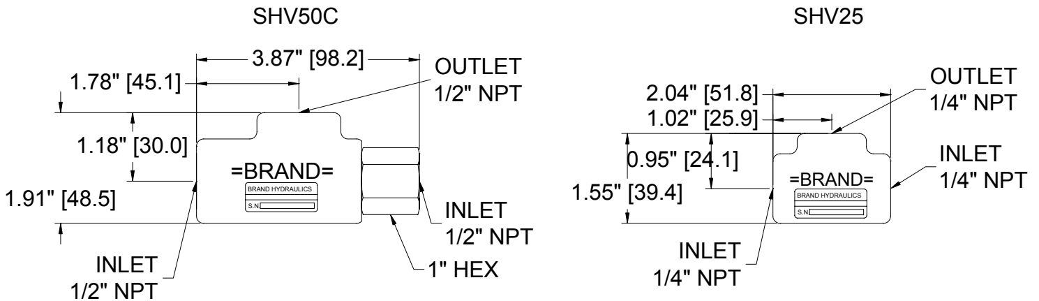
Figure 1: Dimensional Data for SHV style valves in inches & [millimeters].
