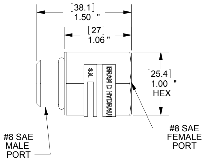
Figure 1: Dimensional Data for 84AFF style valves in inches & [millimeters].
