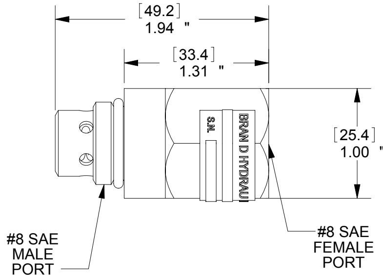
Figure 1: Dimensional Data for 83AFF style valves in inches & [millimeters].
