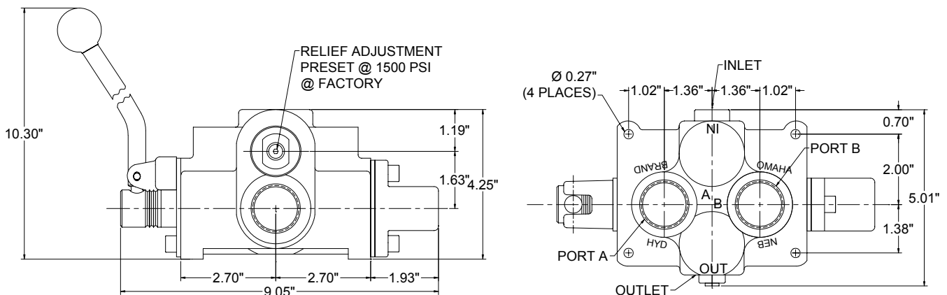
Figure 1: Dimensions for DCF valve, L-style handle shown in standard position
