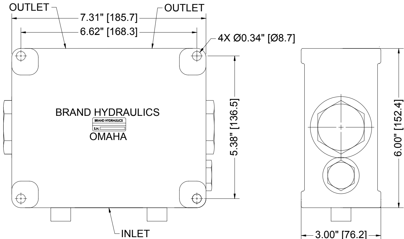
Figure 1: Dimensional Data for B100-24SAE valve in inches & [millimeters].
